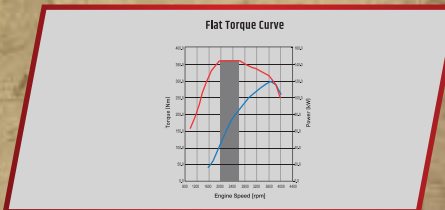
Flat Torque Curve
